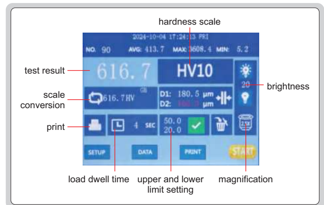
Vickers measurement interface
