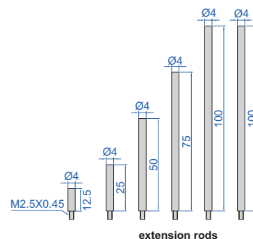
extension rods
