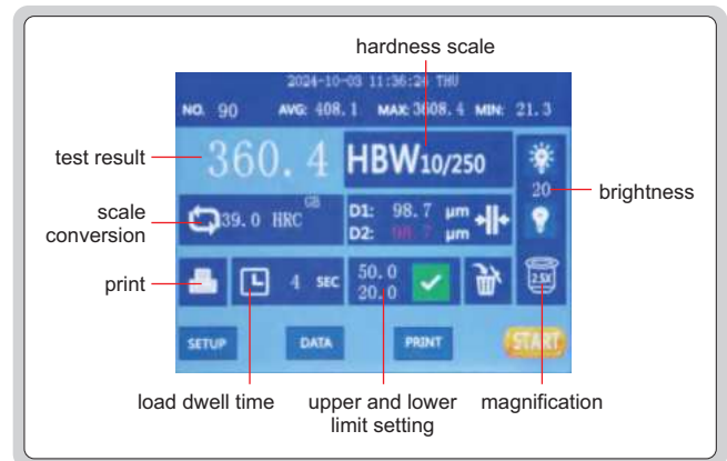
Brinell measurement interface
